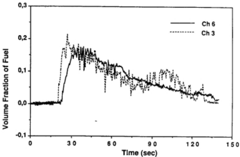
Figure 2 Concentration profiles measured at probe locations C3 and C6 for a test releasing methane from a 20 mm orifice (initial tank pressure 10 bar). The release was pointed upwards. A 0.6 m/s wind was blowing through the module.
